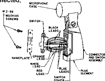
MODEL 548S — IMPEDANCE SELECTION
