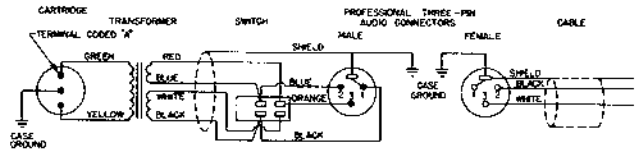
MODEL 548S — INTERNAL CONNECTIONS
