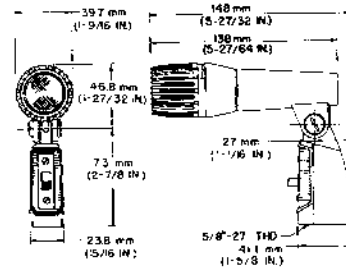
MODEL 548S — OVERALL DIMENSIONS FIGURE 3
