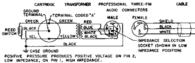
MODELS 548SD AND 548SD-CN INTERNAL CONNECTIONS
