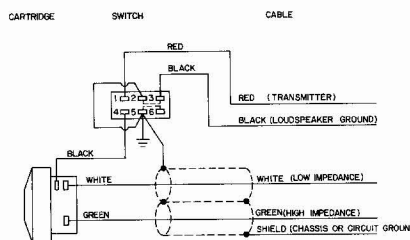
INTERNAL CONNECTIONS FIGURE 1
