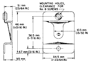
MOUNTING BRACKET FIGURE 3
