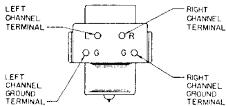
TERMINAL DIAGRAM
