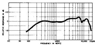
TYPICAL FREQUENCY RESPONSE FIGURE 1
