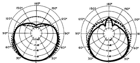
TYPICAL POLAR PATTERNS FIGURE 2
