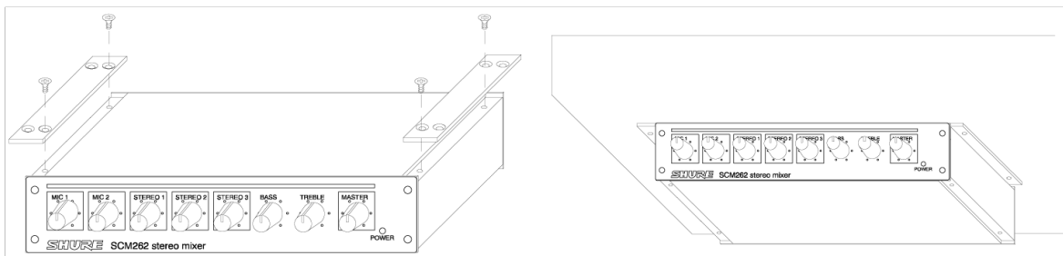
Hanging Mount
