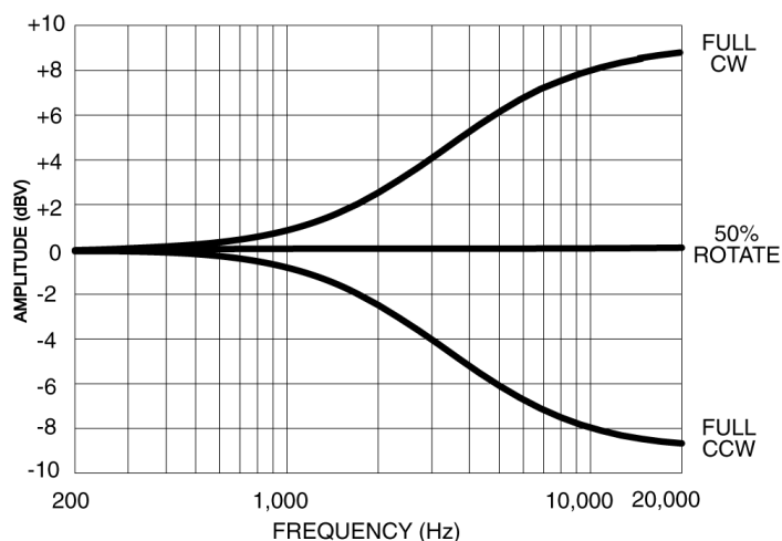
HIGH-FREQUENCY SHELIVING EFFECTS
