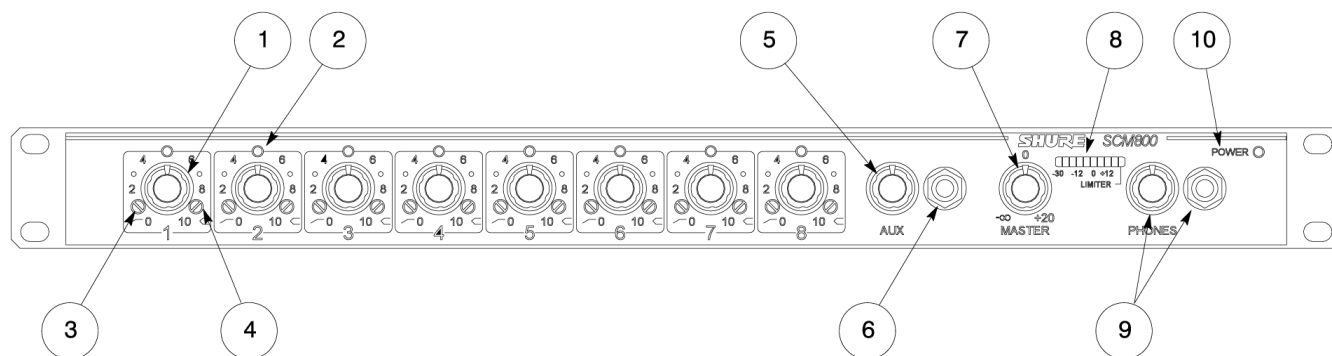
MODEL SCM800/E FRONT PANEL FIGURE 1
