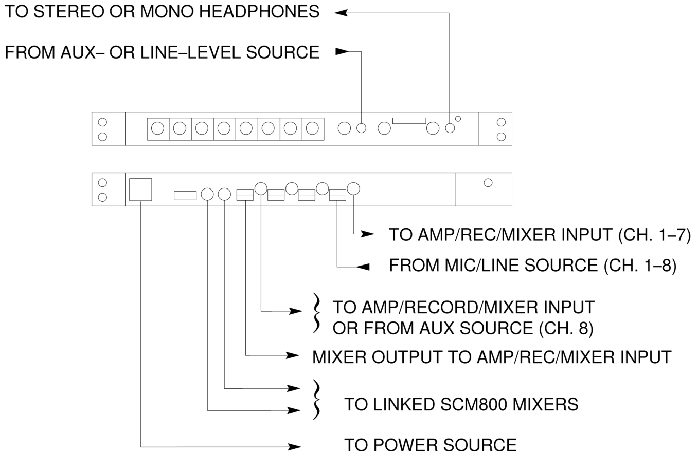
SCM800/E AUDIO CONNECTIONS FIGURE 5
